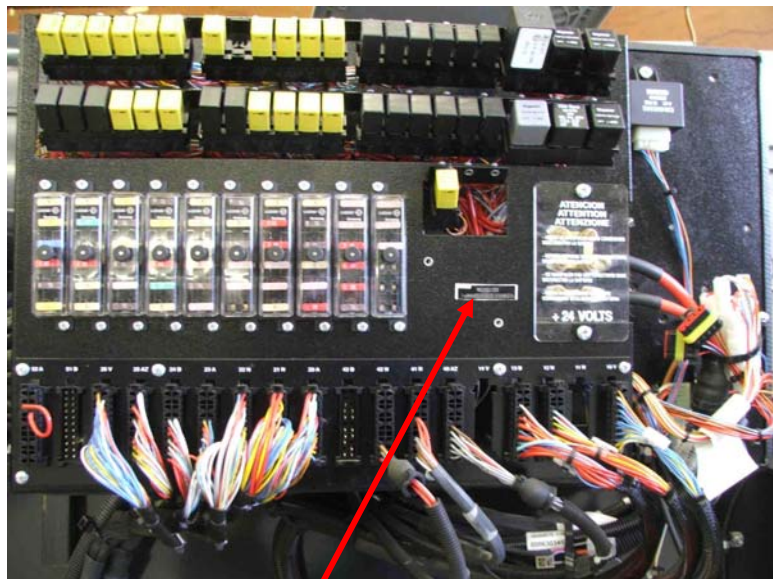
Left hand junction board (use clear fluid)
