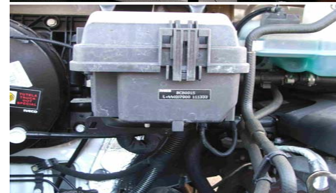
Fuse and Relay Box (use clear fluid)
